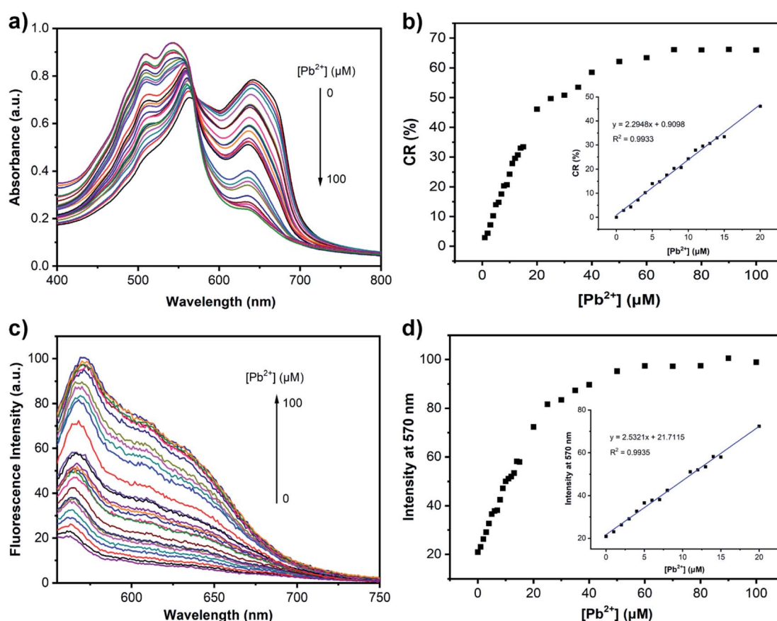
Fig. 5 (a) UV-vis absorption spectra and (b) related CR (%) values of PDA-EDEA-TAA liposomes (100 \mu\text{M} ) in HEPES buffer (10 mM, pH = 7.4) with the increasing concentration of \text{Pb}^{2+} ions (0–100 \mu\text{M} ) at room temperature. Inset: the linear relationship between the CR (%) value of PDA-EDEA-TAA liposomes and \text{Pb}^{2+} concentrations. (c) Fluorescence emission spectra and (d) related fluorescence intensity changes at 570 nm of PDA-EDEA-TAA liposomes (100 \mu\text{M} ) in HEPES buffer (10 mM, pH = 7.4) upon the addition of different concentrations of \text{Pb}^{2+} ions (0–100 \mu\text{M} ) at room temperature. Inset: the linear relationship between the fluorescence intensity of PDA-EDEA-TAA liposomes and \text{Pb}^{2+} concentrations.
