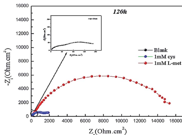
Fig. 10 Nyquist plots of the Cu obtained in 1 M \text{HNO}_3 solution in the absence and containing 1 mM Cys or 1 mM L-Met after 120 h.
