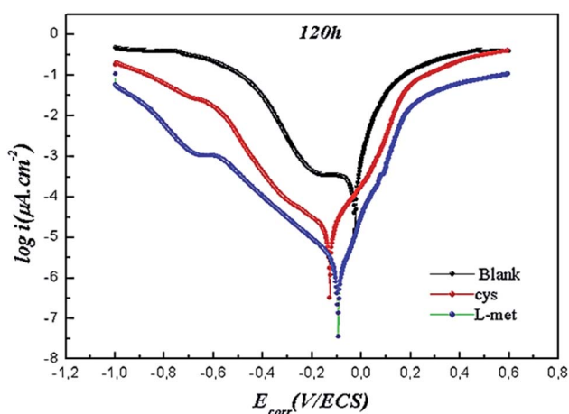
Fig. 9 Potentiodynamic polarization curves of Cu after exposing to 1 M \text{HNO}_3 solution in the absence and presence of 1 mM Cys or 1 mM L-Met for 120 h immersion.
