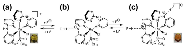
Scheme 1 Two NH groups of each Hdpa ligands in cis -[RuCl(dms \bar{o} -S)(Hdpa) _2 ] ^+ [structure (a)] reacted with added F^- anions to form cis -[RuCl(dms \bar{o} -S)(FHdpa) _2 ] ^- [structure (c)] via cis -[RuCl(dms \bar{o} -S)(FHdpa)(Hdpa)] [structure (b)]. The solution of the original complex was yellow, and after adding the F^- anions, it turned orange. Li ^+ was added to the orange solution and it returned to the original yellow color recovering cis -[RuCl(dms \bar{o} -S)(Hdpa) _2 ] ^+ [structure (a)] and LiF.
