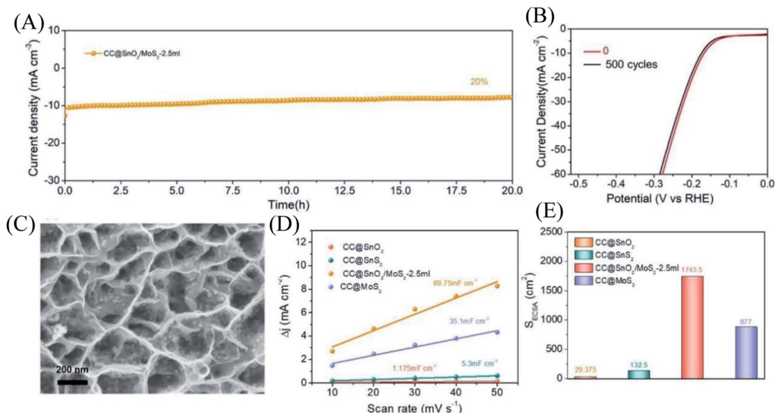
Fig. 4 (A) Curve of i-t with a constant current density of 10 \text{ mA cm}^{-2} . (B) LSV curve comparison of the \text{SnO}_2/\text{MoS}_2 NS-2.5 sample in 0 cycle and 500 cycles. (C) SEM image of \text{SnO}_2/\text{MoS}_2 NS-2.5 sample after 500 cycles. (D) The curve between CV scanning rate and current density of each sample. (E) The electrochemical active area of each sample.
