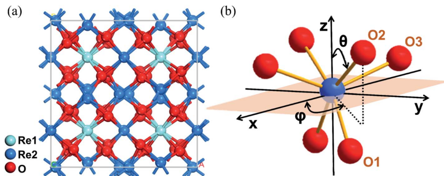
Fig. 1 (a) Structure of the \text{Yb:Lu}_x\text{Y}_{2-x}\text{O}_3 crystal. (b) Coordination octahedron composed of the Re2-site ion and surrounding oxygen ions in the polar coordinate system. \theta and \varphi represent the polar and azimuth angles of each oxygen ion relative to the origin of the coordinates, respectively.
