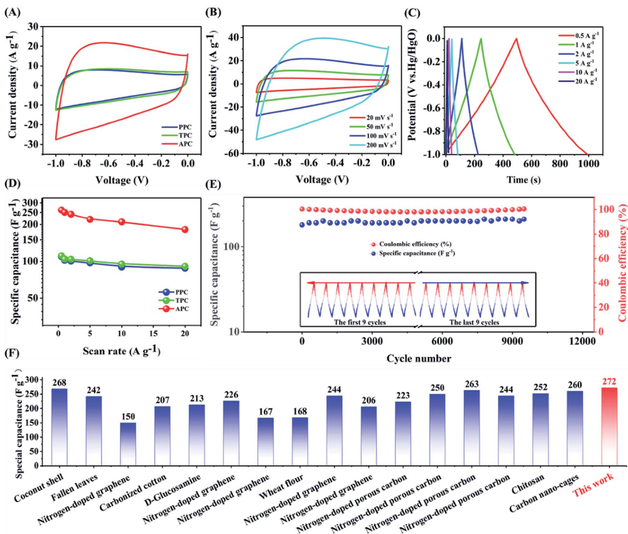
Fig. 4 (A) CV curves of PPC, TPC and APC electrodes at a scan rate of 100 \text{ mV s}^{-1} . (B) CV curves of APC at different scan rates of 20, 50, 100, and 200 \text{ mV s}^{-1} in 6.0 M KOH aqueous solution. (C) Galvanostatic charge/discharge curves of APC at various current densities. (D) Specific capacitances of PPC, TPC, and APC at different current densities. (E) Electrochemical stability of APC for 10 000 cycles tested at 200 \text{ mV s}^{-1} . (F) Comparison of the specific capacitance of APC with that of other sugars (Table 4S † ).
