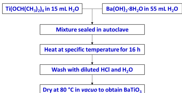
Scheme 1 Hydrothermal synthesis to prepare \text{BaTiO}_3 , using various Ba/Ti precursor ratios/concentrations and reaction temperatures.
