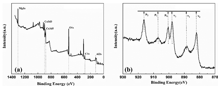
Fig. 8 (a) The XPS survey spectrum of CeO 2 /MgAl-LDO(P123); (b) the Ce 3d spectrum.
