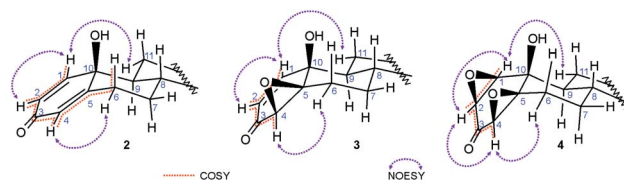
Fig. 2 1 H– 1 H COSY and NOE correlations in quinols 2 , epoxyquinols 3 and diepoxides 4 . COSY couplings: vinylic (H–C(1)–H–C(2)), W (H–C(2)–H–C(4)) and allylic (H–C(4)–H \beta –C(6)).
