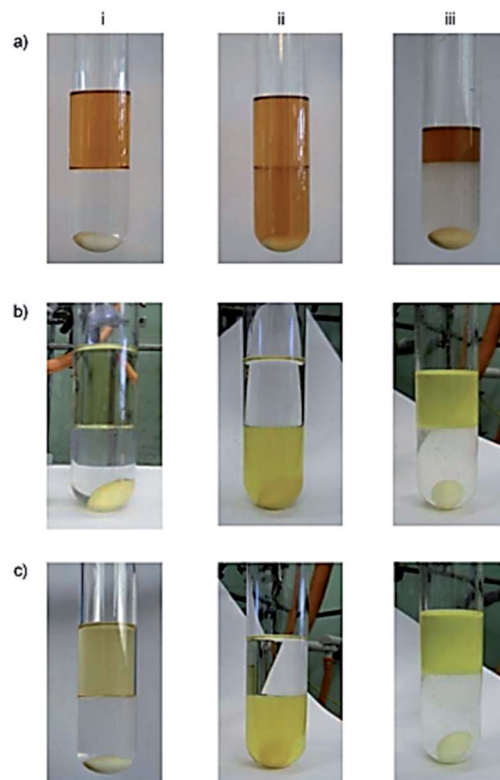
Fig. 20 Phase switching after the hydroformylation of 1-octene catalyzed by rhodium complexes of (a) 2; (b) 2 and 1 combined, cycles 1a and 1b; (c) 2 and 1 combined, cycle 2. (i) Reaction solution with water added. (ii) After bubbling \text{CO}_2 through the mixture for 1.5 h. (iii) After phase separation, addition of fresh toluene, and bubbling \text{N}_2 through the mixture at 60°C for 1.5 h. The top (organic) phase from (b iii) was used for the hydroformylation of 1-octene to give the product phase shown in (c i). Reprinted by permission from ref. 31, Copyright © 2012 WILEY-VCH Verlag GmbH & Co. KGaA, Weinheim.
