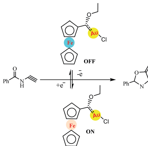
Scheme 31 Switchable gold-catalysed cyclisation of N(2\text{-propyn-1-yl})\text{benzamide} to 2-phenyl-5-vinylidene-2-oxazoline. Reprinted by permission from ref. 82, Royal Society of Chemistry.
