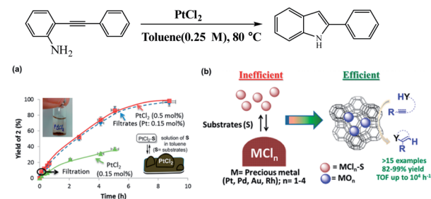
Fig. 18 (a) Yield–time profile for the hydroamination of o -(phenylacetylen)aniline catalyzed by PtCl 2 . The photograph on the left shows the precipitate of PtCl 2 in toluene under reaction conditions, and the illustration on the right describes the equilibrium-controlled dissolution of PtCl 2 with substrates under reaction conditions. (b) Schematic illustration using metal-exchanged zeolite as substitute catalysts for hydroamination reactions with high activity. Reprinted by permission from ref. 100, Copyright © 2015, American Chemical Society.
