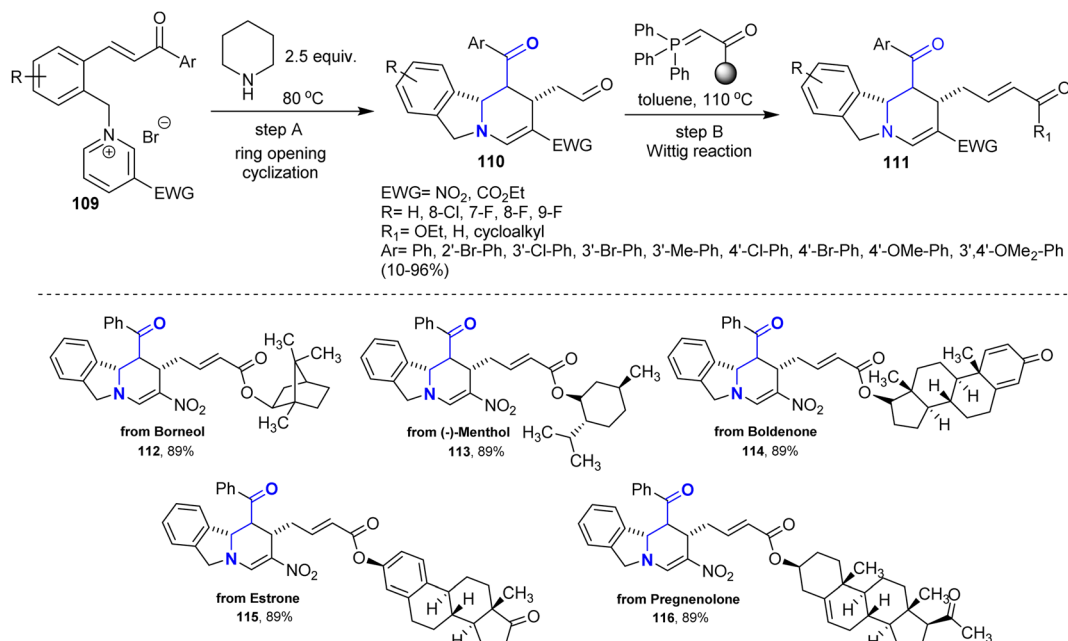
Scheme 39 Synthesis of tetrahydropyrido-isoidoles.
