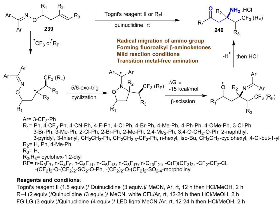
Scheme 58 Synthesis of \beta -aminoketones through amination and radical migration of amino group.
