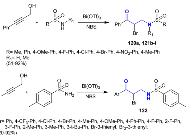
Scheme 41 Synthesis of α-bromo-β-aminoketones.
