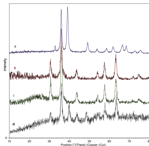
Fig. 6 The X-ray diffraction (XRD) pattern of (a) CuO QDs, (b) \text{Fe}_3\text{O}_4 , (c) M-MSNs and (d) M-MSNs/CuO(QDs).
