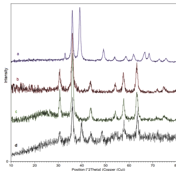
Fig. 6 The X-ray diffraction (XRD) pattern of (a) CuO QDs, (b) Fe 3 O 4 , (c) M-MSNs and (d) M-MSNs/CuO(QDs).
