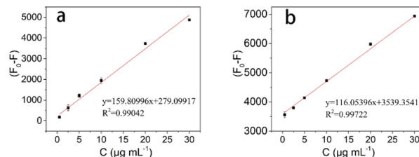
Fig. 5 The linear relationship between (F_0 - F) of CDs-MIPs (a), CDs-NIPs (b) and concentrations of TC (0.5, 2.5, 5, 10, 20, 30 \mu\text{g mL}^{-1} ). F_0 and F indicate the fluorescence intensity signals with and without TC, respectively.
