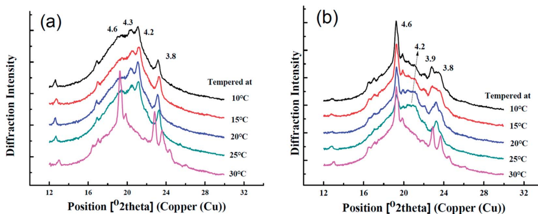
Fig. 5 XRD of samples A and B tempered at 10 °C, 15 °C, 20 °C, 25 °C, and 30 °C.
