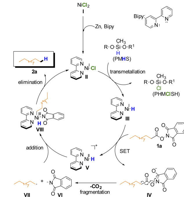
Scheme 2 Proposed mechanism.
