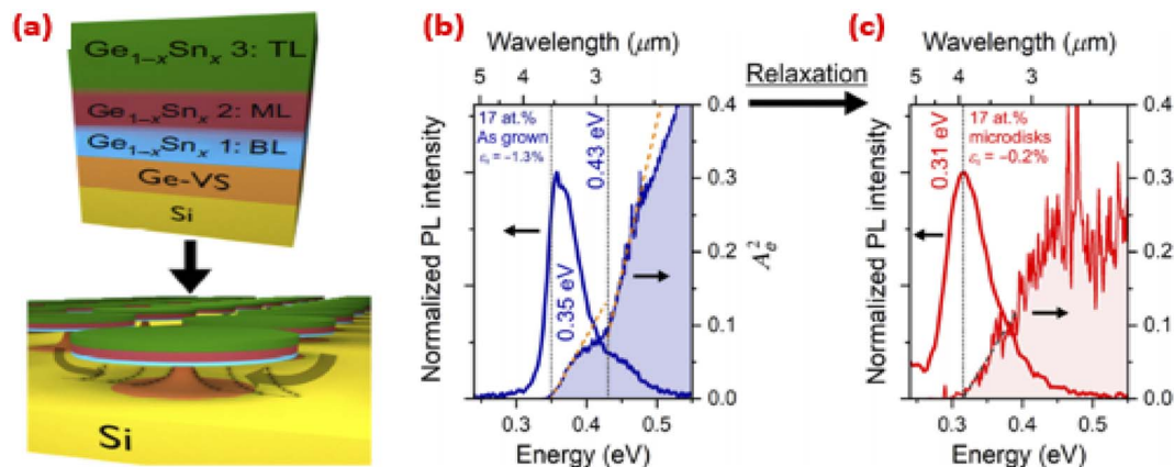
Fig. 19 Ge 1-x Sn x multilayer with different Sn content heterostructures and its PL emission. "Reproduced from ref. 86 with permission from [American Physical Society publisher], copyright [2021]".
