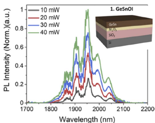
Fig. 20 Ge 0.94 Sn 0.06 layer was grown on the insulating oxide layer and the PL emission at different pumping powers. "Reproduced from ref. 87 https://opg.optica.org/oe/fulltext.cfm?uri=oe-29-18-28959&id=458147 CC BY 4.0".
