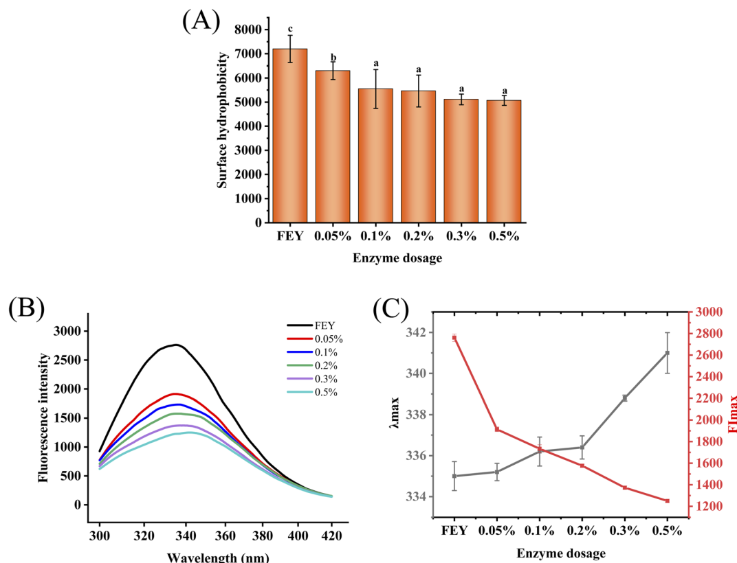
Fig. 5 Surface hydrophobicity (A), fluorescence spectra (B), F_{lmax} and \lambda_{max} (C) of hydrolysed egg yolk modified with different enzyme dosages. Different letters indicate significant differences ( p < 0.05 ).
