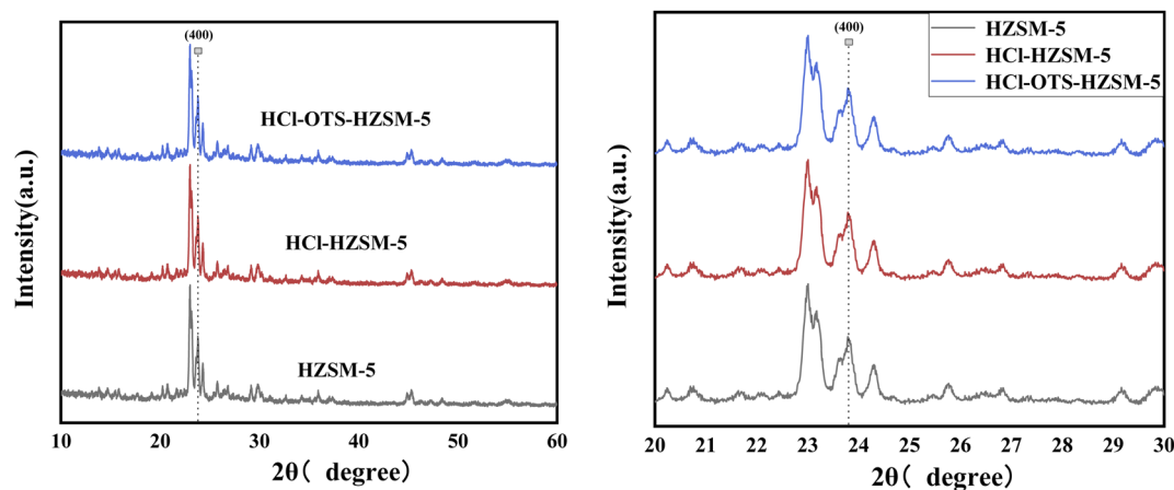
Fig. 3 XRD patterns of HZSM-5, HCl-HZSM-5 and HCl-OTS-HZSM-5 zeolites.
