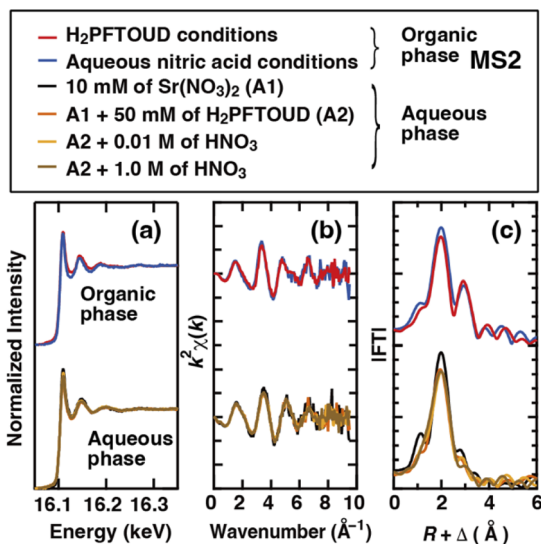
Fig. 10 Normalized Sr K-edge XAFS spectra (a), k^2 -weighted Sr K-edge EXAFS spectra (b), and Fourier transform data (c) obtained for each phase under \text{H}_2\text{PFTOUD} and aqueous nitric acid conditions.
