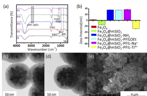
Fig. 1 Structural characterizations of nanoparticles. (a) FT-IR spectra of \text{Fe}_3\text{O}_4 (i), \text{Fe}_3\text{O}_4@m\text{SiO}_2 (ii), \text{Fe}_3\text{O}_4@m\text{SiO}_2\text{-NH}_2 (iii), \text{Fe}_3\text{O}_4@m\text{SiO}_2\text{-PFILOEt} (iv), and \text{Fe}_3\text{O}_4@m\text{SiO}_2\text{-PFIL-Ti}^{4+} (v). (b) Zeta potentials of \text{Fe}_3\text{O}_4 , \text{Fe}_3\text{O}_4@m\text{SiO}_2 , \text{Fe}_3\text{O}_4@m\text{SiO}_2\text{-NH}_2 , \text{Fe}_3\text{O}_4@m\text{SiO}_2\text{-PFILOEt} , \text{Fe}_3\text{O}_4@m\text{SiO}_2\text{-PFIL-Na}^+ , and \text{Fe}_3\text{O}_4@m\text{SiO}_2\text{-PFIL-Ti}^{4+} . TEM images of (c) \text{Fe}_3\text{O}_4@m\text{SiO}_2 and (d) \text{Fe}_3\text{O}_4@m\text{SiO}_2\text{-PFIL-Ti}^{4+} . (e) SEM image of \text{Fe}_3\text{O}_4@m\text{SiO}_2\text{-PFIL-Ti}^{4+} .
