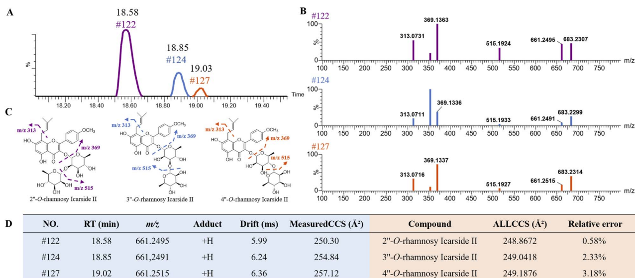
Fig. 7 Characterization of isomers with m/z 661.2496 and CCS prediction based on ALLCCS platform. (A) Three peaks extracted ion chromatography (EIC) of m/z 661.2495 [M + H]^+ , (B) MS/MS spectra of three compounds (peak 122, 124 and 127), (C) fragmentation behaviors of 2''-O-rhamnosy icarside II, 3''-O-rhamnosy icarside II and 4''-O-rhamnosy icarside II, (D) the RT, measured molecular weight, adducts, drift time, measured experimental CCS values and their predicted CCS values from ALLCCS platform of three compounds. Relative error represents the accuracy between measured experimental CCS values and predicted CCS values.
