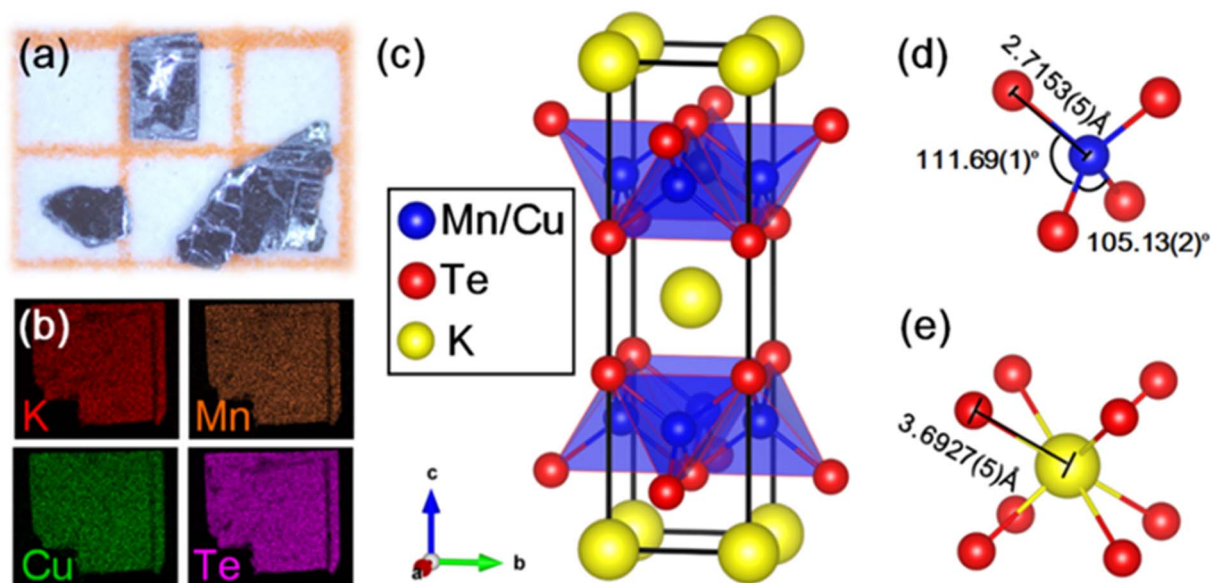
Fig. 1 (a) Optical photograph of the single-crystal sample of KMnCuTe 2 . (b) Elemental mapping of the sample. (c) Crystal structure of KMnCuTe 2 with tetragonal I4/mmm space group. The detailed bond lengths and angles in (d) [Mn(Cu)Te 4 ] tetrahedron and (e) [KTe 8 ] cube.
