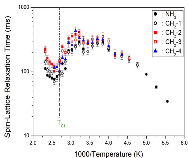
Fig. 9 ^1\text{H} NMR spin–lattice relaxation times of \text{NH}_3 and \text{CH}_2 in [\text{NH}_3(\text{CH}_2)_6\text{NH}_3]\text{ZnBr}_4 as a function of inverse temperature.
