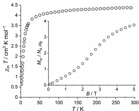
Fig. 7 Temperature dependence of \chi_m T at 1.0 T of 2 ; inset: field dependence of the molar magnetization M_m at 2.0 K.
