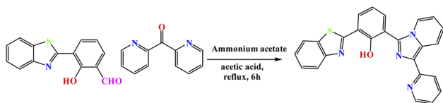
Scheme 1 The synthetic route of sensor BIPP.
