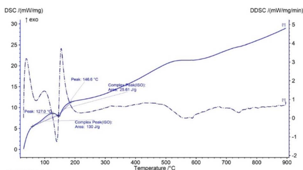
Fig. 2 Differential scanning calorimetry (DSC) analysis of the raw sample (gypsum).
