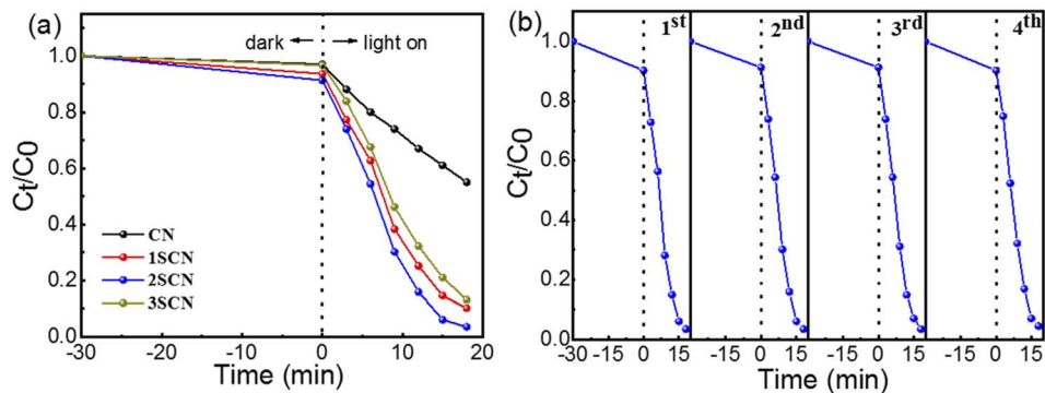
Fig. 7 Photocatalytic degradation of RhB (a) under visible light irradiation. (b) Stability of 2SCN.
