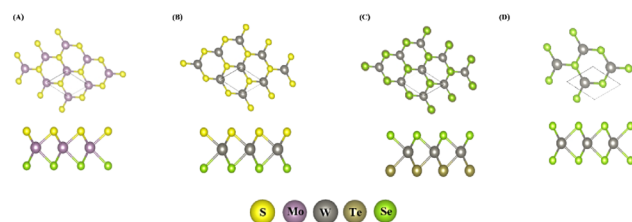
Fig. 1 Top and side views of (A) MoSse, (B) WSe, (C) WSeTe, and (D) WSe 2 monolayers.
