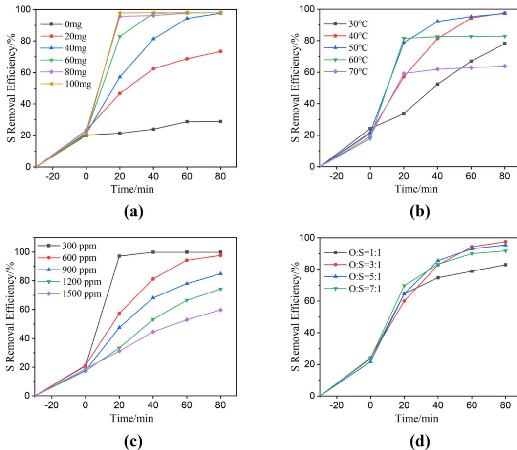
Fig. 3 Catalytic oxidative desulfurization of NiCo 2 O 4 powders at different experimental conditions ((a) NiCo 2 O 4 dosage; (b) temperature; (c) DBT initial dosage; (d) O : S ratio).
