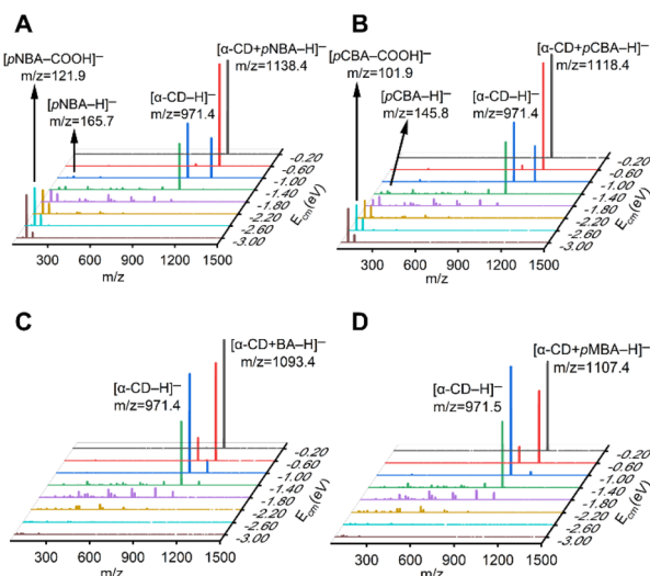
Fig. 1 Tandem mass spectra of the (A) [\alpha\text{-CD} + p\text{NBA-H}]^- , (B) [\alpha\text{-CD} + p\text{CBA-H}]^- , (C) [\alpha\text{-CD} + \text{BA-H}]^- and (D) [\alpha\text{-CD} + p\text{MBA-H}]^- complex anions with increasing E_{\text{cm}} .
