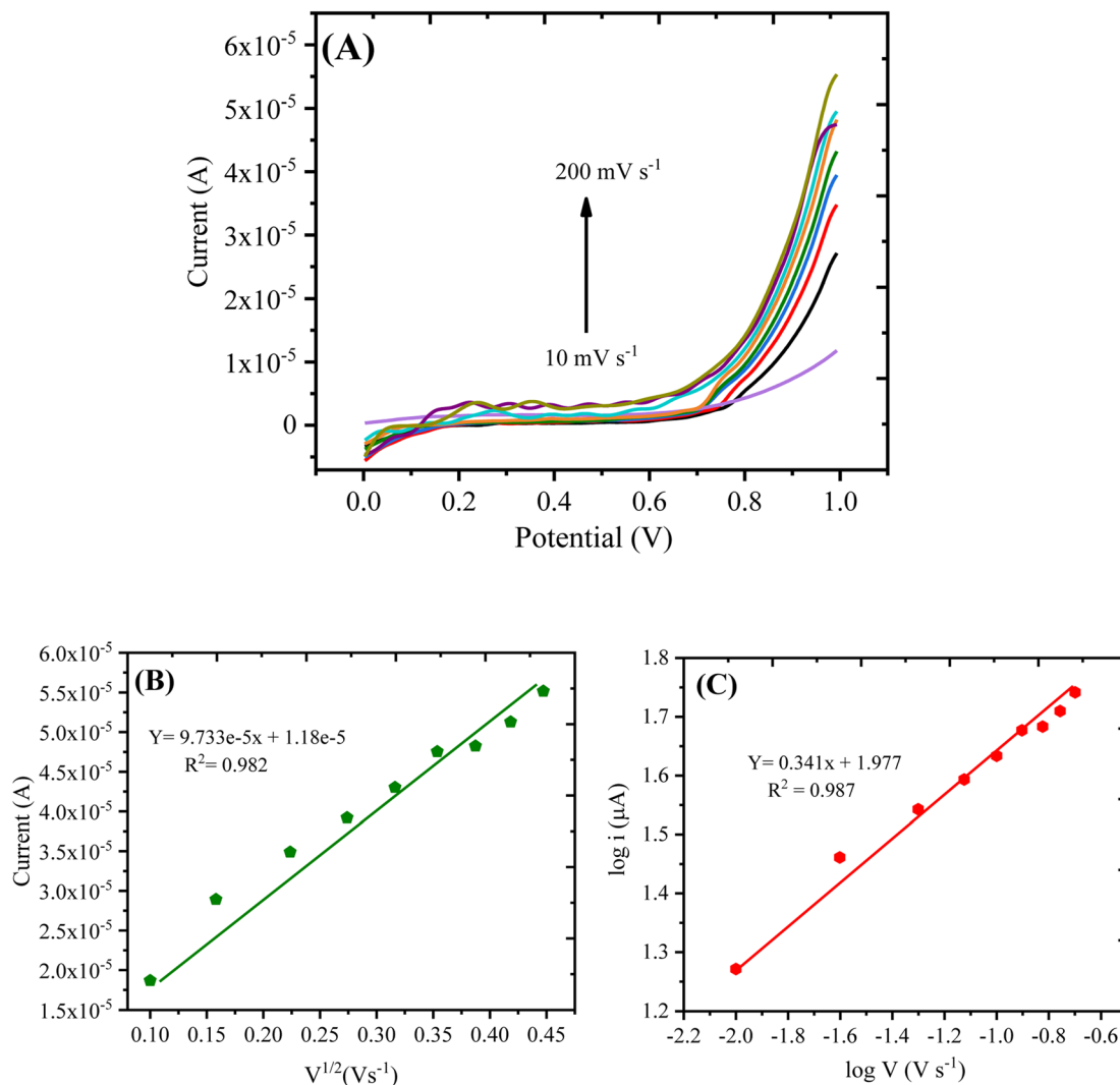
Fig. 8 (A) LSV curve showing the scan rate effect on the oxidation current of 0.1 mM H 2 O 2 . (B) Oxidation current plotted against v 1/2 and (C) the logarithm of the oxidation current plotted against the logarithm of the scan rate.
