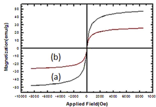
Fig. 6 VSM images of (a) Fe 3 O 4 and (b) nano-cellulose/Ti (IV) /Fe 3 O 4 .
