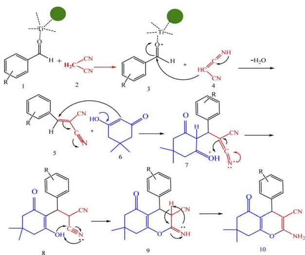
Scheme 1 A plausible mechanism for synthesis of chromenes in the presence of nano-cellulose/Ti (IV) /Fe 3 O 4 .
