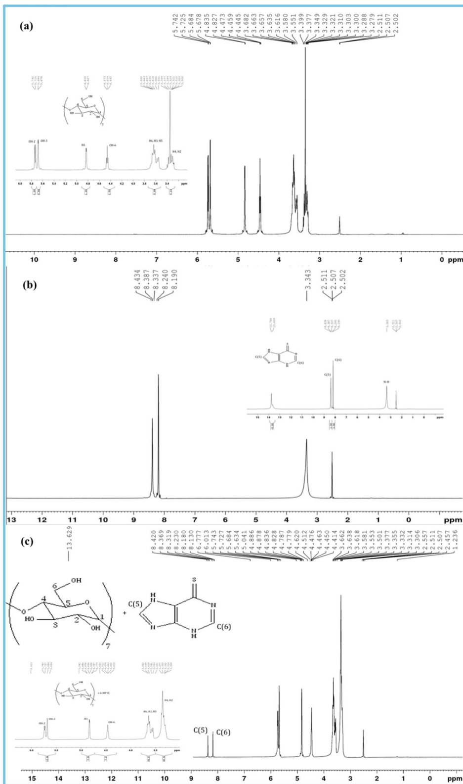
Fig. 4 1 H NMR spectra of (a) β-CD, (b) 6-MP, and (c) IC.
