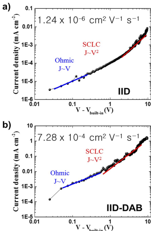
Fig. 4 J–V characteristics of a hole-only device with (a) IID and (b) IID–DAB. The red lines show fits to the Mott–Gurney law in the SCLC regime of device operation.
