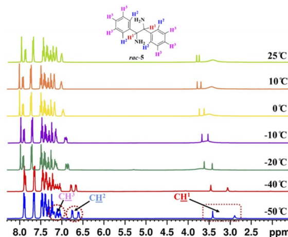
Fig. 3 Partial stacked plot of 1 H-NMR spectrum (400 MHz, CDCl 3 ) of rac - 5 (0.05 mmol) with ( S )- 3a (0.1 mmol) at variable temperatures in chloroform- d (0.6 mL). CH 1 , CH 2 , and CH 3 resonances are highlighted in wine red colour box.
