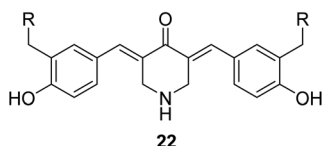
Fig. 10 3,5-Bis(hydroxyarylidene)-4-piperidones 22 with alkylamino-methyl substituents.
