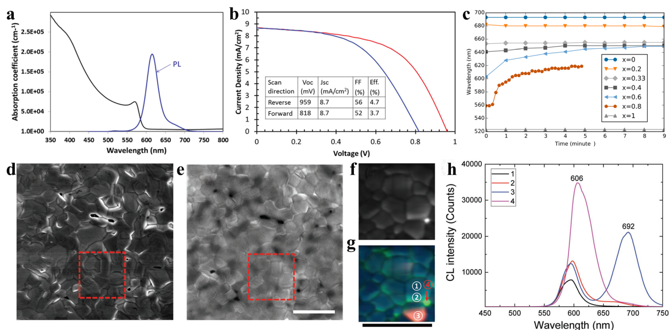
Fig. 8 (a). Absorption coefficient and steady-state PL spectrum of CsPbI_{2-x}Br_x sample. (b). J-V curves of the best-performing CsPbI_{2-x}Br_x cell. (a and b) Reproduced with permission. 33 Copyright 2016, Wiley-VCH. (c). PL peak position as a function of time for CsPb(Br_xI_{1-x})_3 materials under \sim 1 sun illumination. Reprinted with permission. 44 Copyright 2016, the American Chemical Society. (d) Secondary electron SEM image and (e) CL PMT mapping of the CsPbI_{2-x}Br_x film ( 1024 \times 1024 pixels ( \approx 11 nm on a side); dwell time 50 \mu s per pixel) with the electron beam acceleration voltage of 5 kV and current of 799 pA. The square region in d was further studied by CL spectrum mapping with different spectral windows of 530–630 nm (pixel size of 40 nm \times 40 nm; dwell time of 10 ms). (g). Superposition of (f). (h). CL spectra for the area inside a CsPbI_{2-x}Br_x grain (GI; region 1 in (g)), grain boundary (GB; region 2 in (g)), and I-rich phase (areas 3 and 4 in (g)). All the scale bars are 3 \mu m . (d–h) Reproduced with permission. 99 Copyright 2017, Wiley-VCH.
