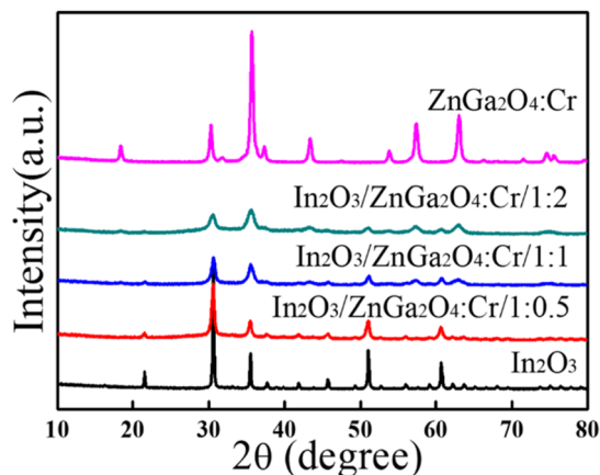
Fig. 2 XRD patterns of the In 2 O 3 , ZnGa 2 O 4 :Cr, and In 2 O 3 /ZnGa 2 O 4 :Cr composites.
