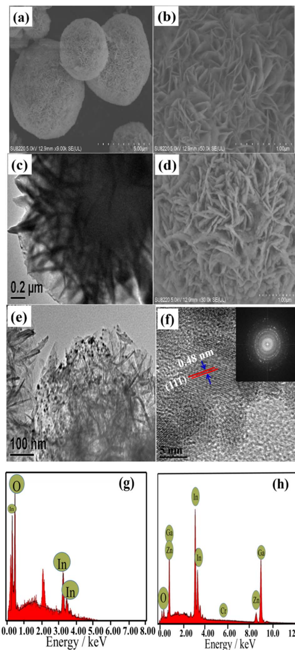
Fig. 3 (a–c) SEM and TEM images of flower-like In 2 O 3 ; (d–f) SEM and TEM, HRTEM, and SAED images of the In 2 O 3 /ZnGa 2 O 4 :Cr/1:1 composites; EDS patterns of the (g) flower-like In 2 O 3 and (h) In 2 O 3 /ZnGa 2 O 4 :Cr/1:1 composites.
