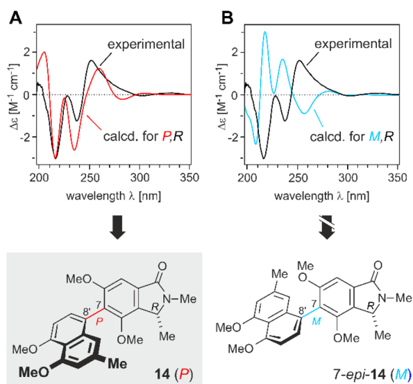
Fig. 4 Assignment of the absolute configuration of ancistrobrevoline A (14) by comparison of its experimental ECD spectrum (in black, taken in methanol) with the ones calculated (A) for the (1R,7P)-isomer (ECD curve in red) and (B) for 1R,7M (in pale blue) using TD \omega B97XD3/def2-TZVP//B3LYP-D3/def2-TZVP.
