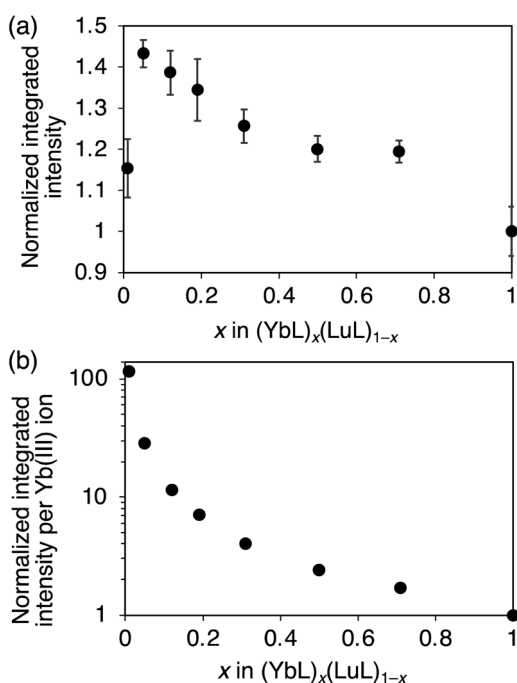
Fig. 4 (a) Normalized integrated intensities of the near-infrared luminescence of (\text{YbL})_x(\text{LuL})_{1-x} and (b) per Yb(III) ion of (\text{YbL})_x(\text{LuL})_{1-x} .
