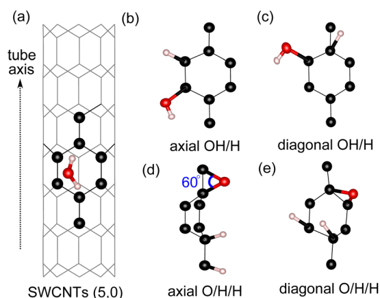
Fig. 2 Surface sites on SWCNT (5,0) for adsorption of: (a) an H_2O molecule, (b) OH/H on the axial C–C site, (c) OH/H on the diagonal C–C site, (d) O/H/H on the axial C–C site and (e) O/H/H on the diagonal C–C site (e).
