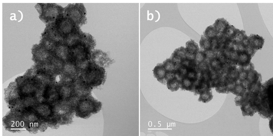
Fig. 9 (a) and (b) BF-STEM images \text{Y}_2\text{O}_2\text{SO}_4:\text{Er,Yb}@\text{AuNPs} precursors hollow spheres. The AuNPs can be observed as small black dots on the surface of the \text{Y}_2\text{O}_2\text{SO}_4:\text{Er,Yb}@\text{AuNPs} hollow spheres.
