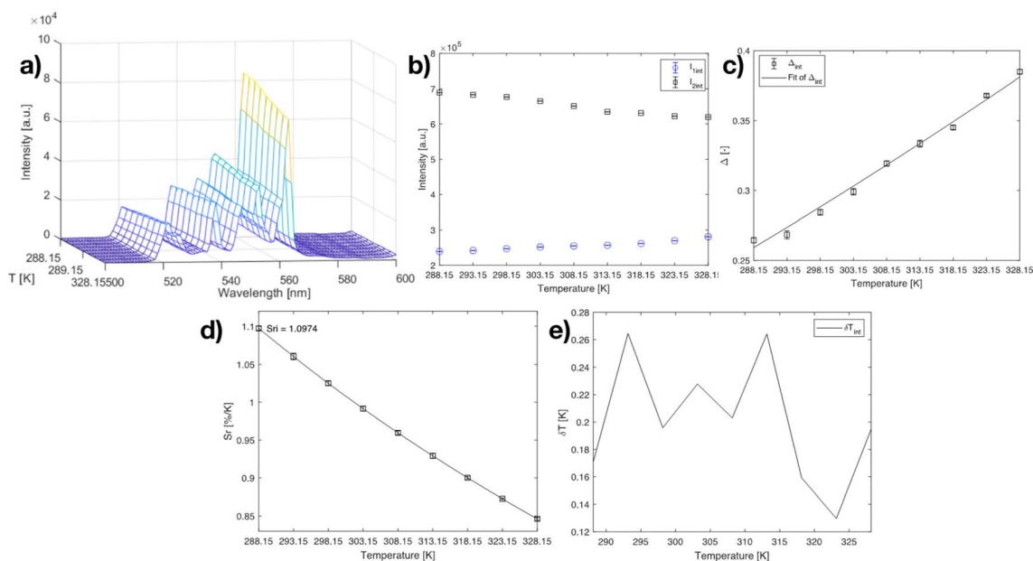
Fig. 7 (a) Emission map of Y_2O_3:Er,Yb at varying temperatures (288.15–328.15 K; step 5 K), (b) intensities of the 522 nm and 563 nm peaks at varying temperatures, (c) calibration curve plot for the Y_2O_3:Er,Yb material using eqn (2) when the 522 nm and 563 nm peaks are considered. The points are experimental \Delta parameters, the solid line shows the least-squares fit to the experimental points. (d) relative sensitivity S_r plot at varying temperatures (288.15–328.15 K) for I_{522}/I_{563} ratio, the solid lines are a guide for the eyes. (e) temperature uncertainty graph over the monitored temperature range.
