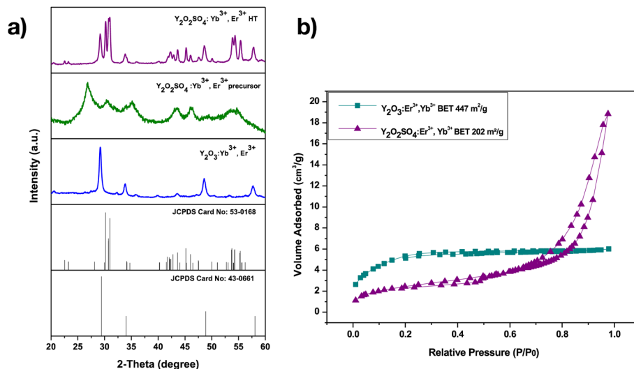
Fig. 6 (a) Powder XRD patterns of Y_2O_3:Er,Yb and Y_2O_2SO_4:Er,Yb (before "precursor" and after heat treatment "HT" at 850 °C for 3 h), (b) N_2 sorption isotherms for Y_2O_3:Er,Yb and Y_2O_2SO_4:Er,Yb precursor.
