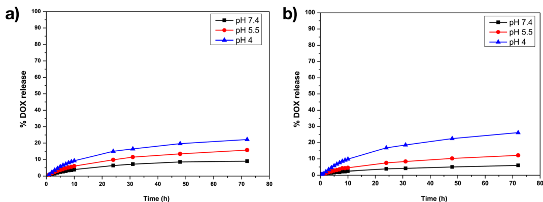
Fig. 11 DOX drug release profiles for (a) Y_2O_3:Er,Yb-DOX , (b) Y_2O_2SO_4:Er,Yb-DOX at pH 7.4, at pH 5.5 and at pH 4 in PBS buffer at 37 °C.
