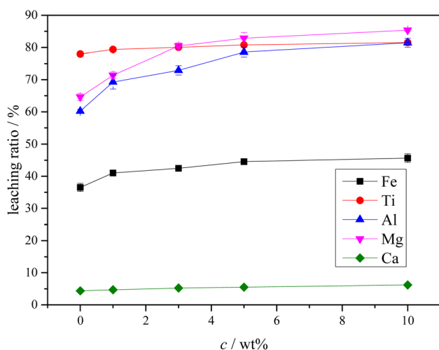
Fig. 8 Effect of sulfuric acid concentration on leaching (liquid-solid ratio: 10 mL g -1 , reaction temperature: 288.15 K (15 °C), reaction time: 60 min).
