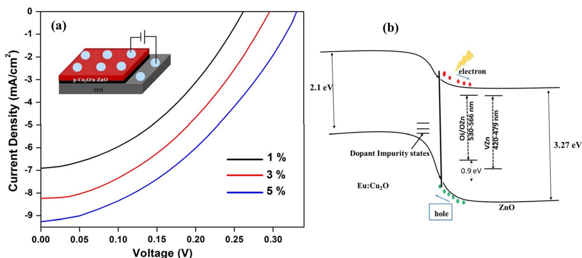
Fig. 18 (a) 1%, 3% and 5% Eu doped thin films having current–voltage characteristics of ITO/ZnO NRs/Eu: Cu 2 O/Al cell, (b) carrier transport and band structure of p–n junction. 129
