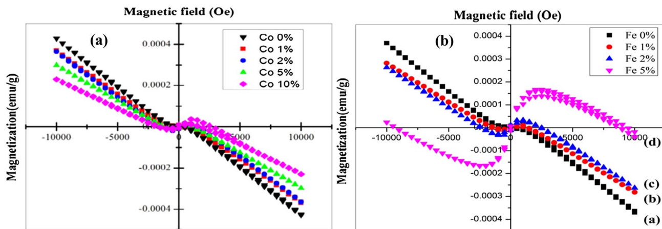
Fig. 19 Magnetic behavior of (a) Co-doped 127 (b) Fe-doped Cu 2 O thin films. 128
