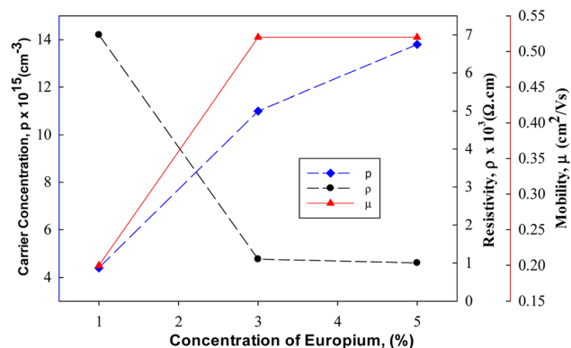
Fig. 17 Resistivity, carrier concentration and mobility for Eu doped Cu 2 O films. 129
