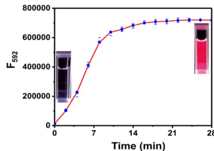
Fig. 3 Time-dependent fluorescence intensity of RHC (10 \mu\text{M} ) with cadaverine (100 \mu\text{M} ). \lambda_{\text{ex}} = 550 \text{ nm} , \lambda_{\text{em}} = 592 \text{ nm} , slits: 2/2 nm. The error bars indicate \pm standard deviation, n = 3 .
