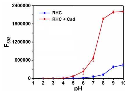
Fig. 4 Fluorescence response of RHC (10 \mu\text{M} ) towards cadaverine (100 \mu\text{M} ) in aqueous solution (DMSO/PBS = 1/9, v/v) with different pH values. \lambda_{\text{ex}} = 550 \text{ nm} , slits: 2/2 nm. The error bars represent \pm SD, n = 3 .
