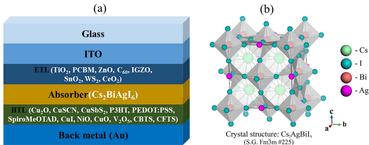
Fig. 1 (a) The design configuration of the Cs 2 AgBiI 6 -based PSC, and (b) the crystal structure of the Cs 2 AgBiI 6 cubic-single-perovskite semiconductor.
