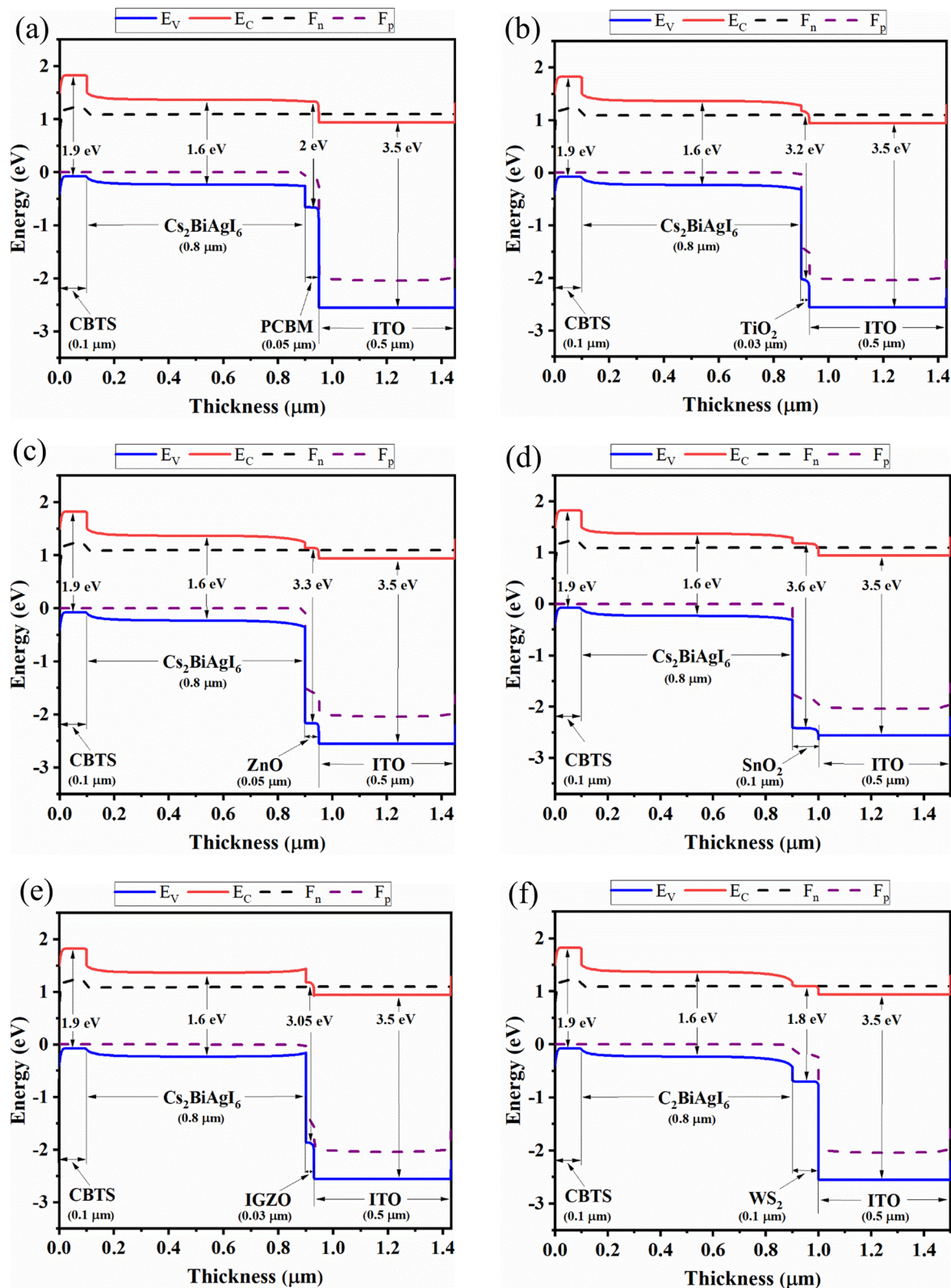
Fig. 5 Energy band diagram of solar cells structure with different ETMs of (a) PCBM, (b) \text{TiO}_2 , (c) \text{ZnO} , (d) \text{SnO}_2 , (e) IGZO, and (f) \text{WS}_2 .
