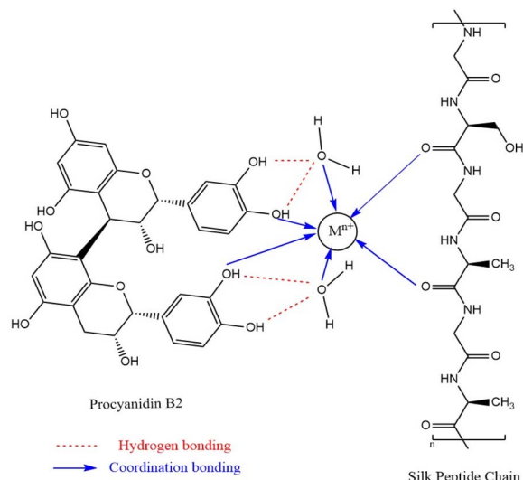
Fig. 6 The possible mordanting mechanism.
