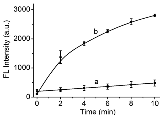
Fig. 3 Fluorescence changes of DCFH-DA in PBS (a) or in the reaction solution (b) of HCH-AcAH (1 \mu\text{M} ) and CES (200 \text{U L}^{-1} ) upon 660 nm laser ( 0.25 \text{ W cm}^{-2} ) for different irradiation time (0–10 min). \lambda_{\text{ex/em}} = 485/525 \text{ nm} .
