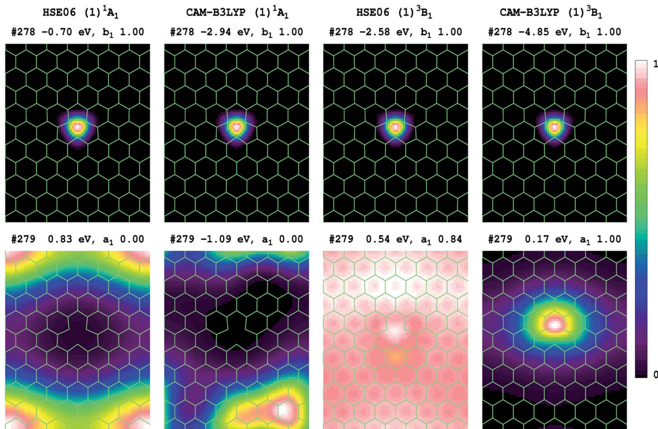
Fig. 3 Shown for of the V_N^{-1} defect in h-BN are the HOMO and LUMO relative electron densities, along a plane 0.8 Å above the atoms, for orbitals #278 and #279 involved in the (1)^3B_1 ( b_1 \rightarrow a_1 ) component of the (1)^3E' lowest-energy state. These are based upon 2D model P_{75} , using 1 \times 2 \times 2 k -points, and list each orbital energy, symmetry, and occupancy (see SI for many more frontier orbitals and analogous results for P_{53} and P_{64} ); for the triplet state, only densities for the spin-up component reflecting the electron majority are shown.
