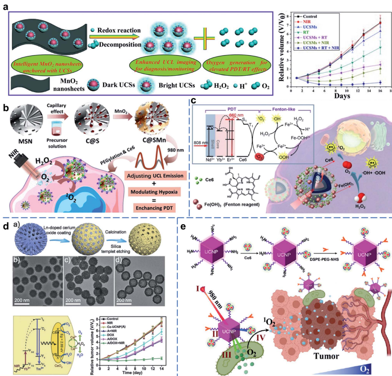
Fig. 4 UCNP-based nanocomposites for O 2 gas therapy. (a) Intelligent MnO 2 nanosheets anchored with UCNs for concurrent pH-/H 2 O 2 -responsive UCL imaging and O 2 -elevated synergistic therapy. 72 (b) UCNP-based nanocomposites for tumor hypoxia modulation and enhanced photodynamic therapy. 78 (c) Ferric hydroxide-modified UCNPs for NIR-triggered synergistic tumor therapy with hypoxia modulation. 79 (d) CeO 2 -modified UCNPs for concurrent pH-/H 2 O 2 -responsive O 2 -evolving synergistic cancer therapy. 83 (e) Cyanobacteria-based NIR-excited self-supplying O 2 system for enhanced photodynamic therapy of hypoxic tumors. 84 Adapted from ref. 72 with permission from Wiley-VCH, copyright 2015; adapted from ref. 78 with permission from American Chemical Society, copyright 2018; adapted from ref. 79 with permission from American Chemical Society, copyright 2018; adapted from ref. 83 with permission from Wiley-VCH, copyright 2018; adapted from ref. 84 with permission from Springer, copyright 2021.
