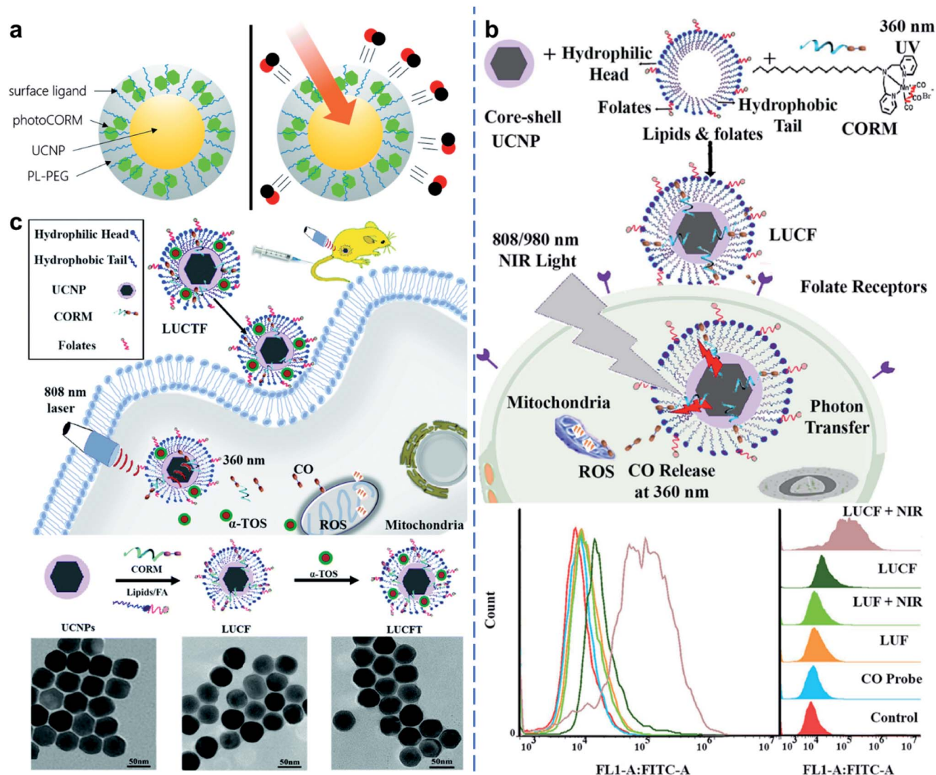
Fig. 8 UCNP-based nanocomposites for CO gas therapy. (a) A photo-activated CO releasing moiety nanocarrier for CO release using NIR light. 37 (b) Lipid-encapsulated UCNPs for NIR-mediated CO release for cancer gas therapy. 100 (c) Vitamin E-facilitated CO pro-drug nanomedicine for efficient light-responsive combination cancer therapy. 101 Adapted from ref. 37 with permission from Royal Society of Chemistry, copyright 2019; adapted from ref. 100 with permission from Elsevier Ltd, copyright 2019; adapted from ref. 101 with permission from Royal Society of Chemistry, copyright 2021.
